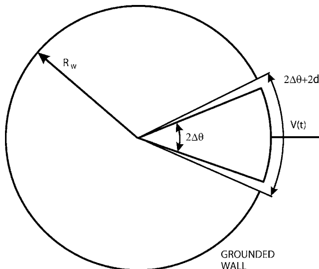
FIG. 7. A schematic of the isolated sector on the trap wall. The angular width of the sector is -\Delta\theta < \phi < \Delta\theta , the gaps are -\Delta\theta - d < \phi < -\Delta\theta and \Delta\theta < \phi < \Delta\theta + d , and the length of the sector is l . In the text, it is assumed that d \ll \theta . A precise calculation of the electric field near the sector should include the gap effects.
