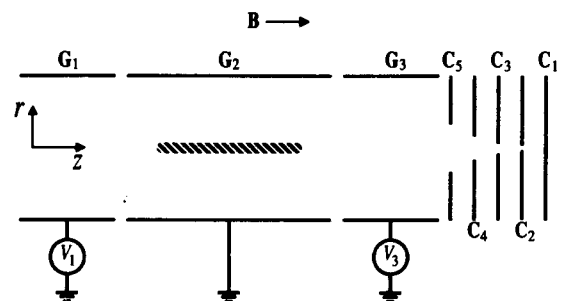
FIG. 1. A schematic of part of the apparatus. The gate radius is R_G = 1.27 cm, and r_3/2 = r_2 = 0.040 cm where r_j is the radius of the hole in collector C_j .
