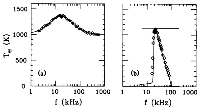
FIG. 2. Experimentally measured T_e vs modulation frequency f (diamonds). (a) Heating comprised of 80 contiguous cycles compared to prediction; (b) heating comprised of 301 sets of 24 cycles, with the total heating process lasting about ten cyclotron radiation times. The horizontal line at T_e=1129 K indicates the temperature of the plasma at the beginning of the heating process.
