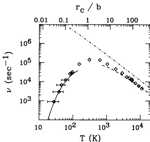
FIG. 3. Measured relaxation rate for B=61.3 kG. The solid curve is the OH prediction. The dashed and dash-dotted curves are plots of the modified IR ( \Lambda=r_c/b ) and the unmodified IR ( \Lambda=\lambda_D/b ) predictions, respectively.
