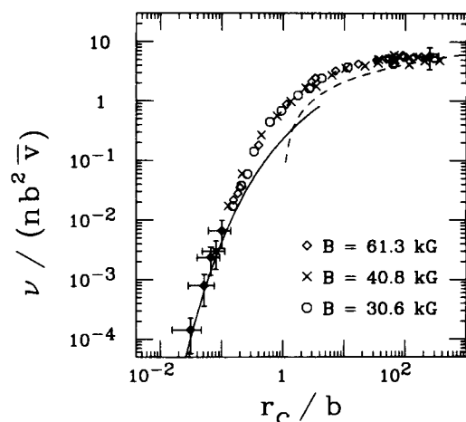
FIG. 4. Normalized rate vs r_c/b . For the \diamond , \times , and \circ data the magnetic fields are 61.3, 40.8, and 30.6 kG, respectively. For all the data \langle n \rangle \approx 8 \times 10^8 \text{ cm}^{-3} . The solid curve is the OH prediction. The dashed curve is the modified IR prediction.
