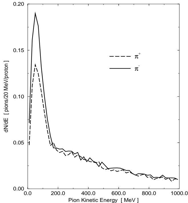
FIGURE 3. ARC energy distribution for 24 GeV protons on Hg.
