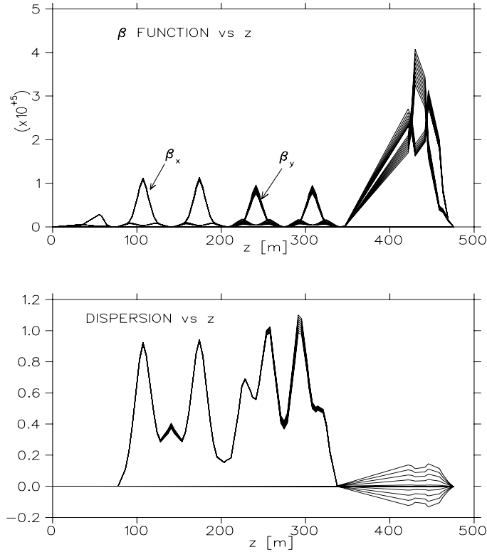
FIGURE 10. Dispersion and \beta functions for different momenta ( \delta p/p = 0.4\% ).
