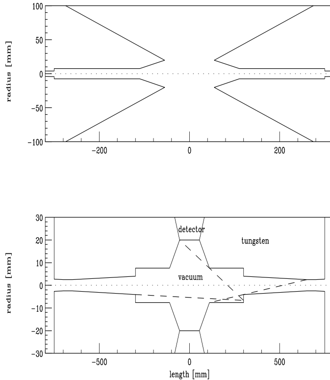
FIGURE 12. Schematic of the detector nose.
