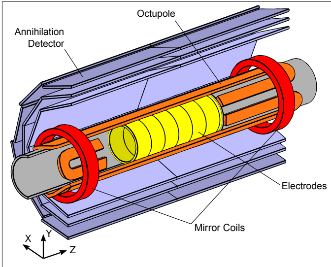
Figure 1: A schematic, cut-away diagram of the antihydrogen production and trapping region of the ALPHA apparatus, showing the relative positions of the Penning-Malmberg electrodes, the minimum-B trap magnets and the annihilation detector. The components are not drawn to scale.
