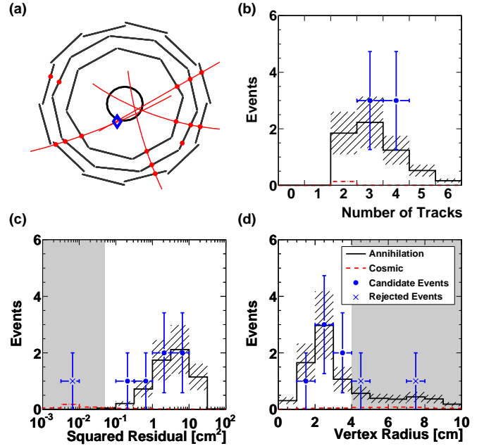
Figure 4: (a) A view of the reconstruction along the z -axis for one of the six events that passed the selection criteria. The elements of this figure have been described in Fig. 2. Comparisons of the events measured in the trapping experiment with the distributions of (b) number of tracks per event (c) squared residual and (d) vertex radial position obtained from applying the selection criteria to the calibration samples. The cut on squared residual and radial position has been ignored in the grey shaded regions excluded by the selection criteria in (c) and (d) respectively. The distributions are obtained by scaling the calibration sample distributions so that the expected number of events, given our data – six for the annihilation data and 0.14 events for the cosmic events – fall inside the acceptance region. The hatch-marked uncertainty regions represent the uncertainties on these numbers. The error bars for the measured events are the counting errors.
