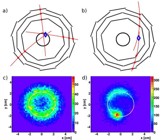
Figure 2: (a) an example reconstruction of an antiproton annihilation and (b) a cosmic ray event. The blue diamond indicates the position of the reconstructed vertex, the red dots the positions of the detected hits, and the inner circle shows the radius of the Penning-Malmberg trap electrodes. (c) The spatial distribution of approximately 2 \times 10^4 antihydrogen atoms identified in this experiment, projected along the z-axis. The distribution is approximately azimuthally uniform and concentrated around the surface of the electrodes, indicated by the white circle. Small non-uniformities are interpreted to be due to the escape of field-ionised antihydrogen (see text). The escape of bare antiprotons tends to produce highly non-uniform distributions, such as that in (d).
