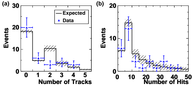
Figure 5: Comparisons of the events measured in the trapping experiment with the distributions of (a) number of tracks per event and (b) number of hits per event, produced by combining the calibration samples with the expected weights (see text). The uncertainties in the distributions are based on the uncertainties in the weighting factors, and the error bars on the data are the counting errors.
