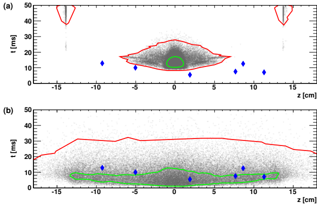
Figure 7: The time after the start of the magnet shutdown and z -position relative to the centre of the trap of the simulated annihilations of (a) mirror-trapped antiprotons and (b) antihydrogen atoms released from the magnetic trap. Individual simulated annihilations are shown as discrete points, of which there are 86914 in (a) and 62438 in (b). The lines show the contours of constant density which contain 50% (green) and 99% (red) of the density when convolved with the resolution of the detector. The solid diamond-shaped points mark the positions of the six surviving events in the trapping experiment. Some mirror-trapped antiprotons impact at \pm 14 cm, where a step in the radius of the electrodes occurs.
