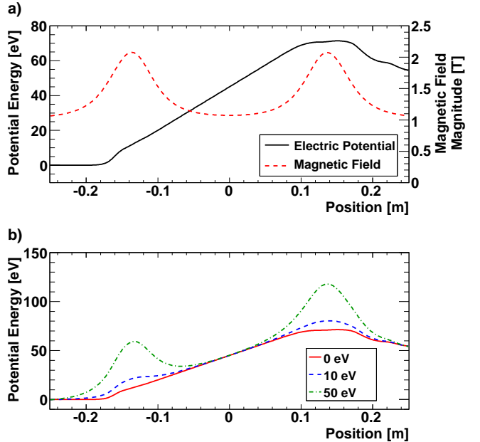
Figure 6: The electric potential (solid line in (a)) and the interaction of the magnetic moment of the antiproton with the inhomogeneous magnetic field (dashed line in (a)) combine to give an E_{\perp} -dependent pseudo-potential on the axis of the trap, three examples of which are shown in (b). Particles with low transverse kinetic energy are not significantly affected by the magnetic fields and are easily cleared from the mixing region. Particles with higher E_{\perp} are the more strongly influenced by the magnetic field and can be confined.
